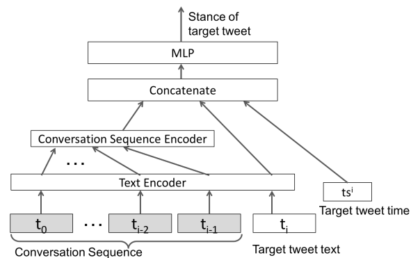
Fig. 3: Architecture of CT-Stance.
